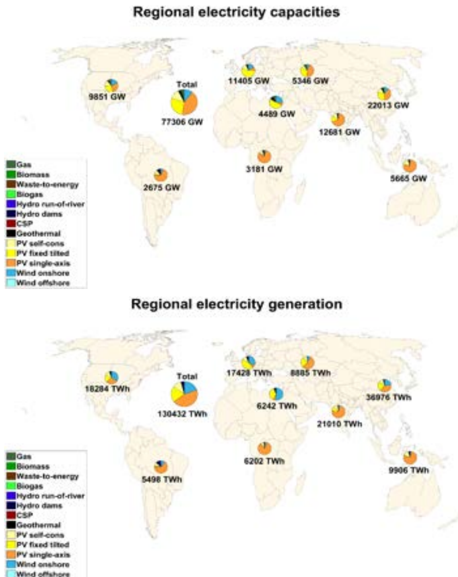
Figure 3.1-25: Global – Regional electricity generation capacities (top) and electricity generation (bottom) in 2050.
