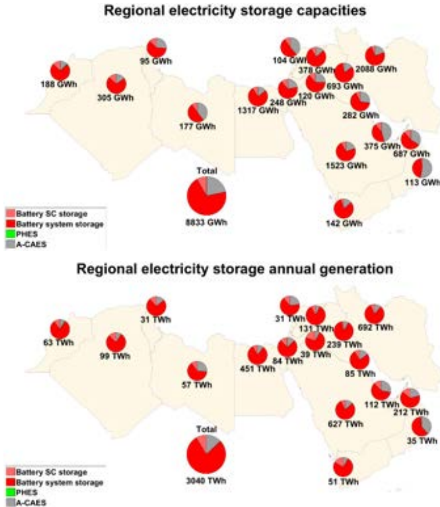
Figure 3.4-28: MENA – Regional electricity storage capacities (top) and electricity storage annual throughput (bottom) in 2050.
