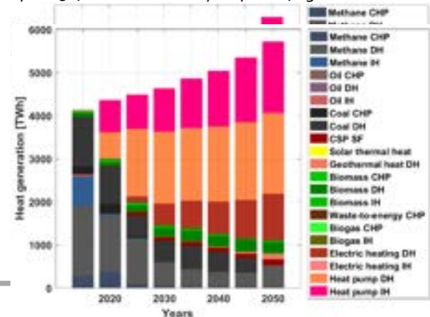
Figure 3.3-8: Eurasia – Primary electricity generation (left) and technology-wise heat generation (right) during the energy transition from 2015 to 2050 in Europe.
