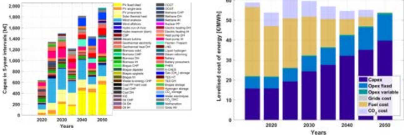
Figure 3.10-7: South America – Capital costs for five-year intervals (left) and levelised cost of energy (right) during the energy transition from 2015 to 2050.
