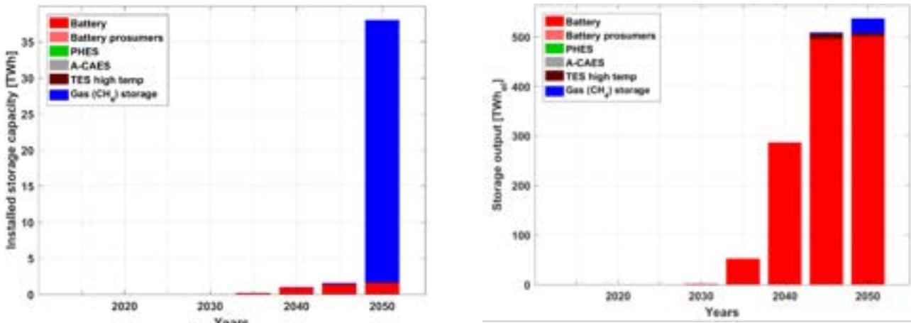
Figure 3.7-23: Northeast Asia – Installed storage capacity (left) and storage output (right) during the energy transition from 2015 to 2050.
