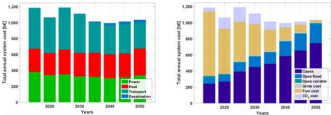
Figure 3.9-6: North America – Annual system costs, sector-wise (left) and functionality-wise (right) during the energy transition from 2015 to 2050.
