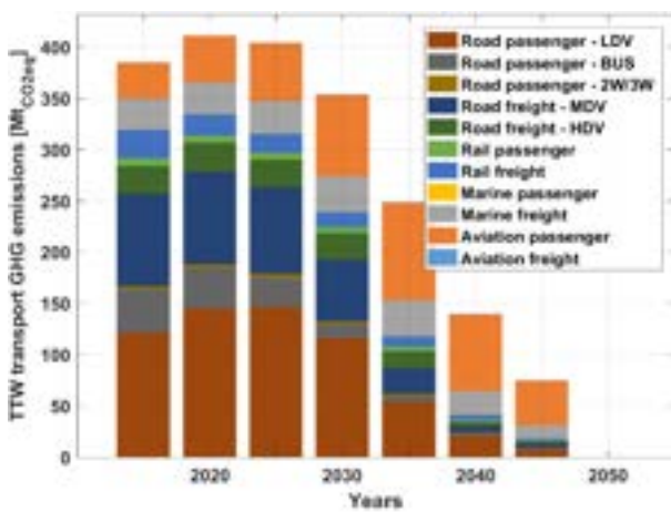
Figure 3.3-32: Eurasia – GHG emissions in the transport sector (left) and GHG emissions in the desalination sector (right) during the energy transition from 2015 to 2050. Tank to Wheel (TTW) considers GHG emissions from readily available fuels and does not consider GHG emissions from the upstream production and delivery of fuels.
