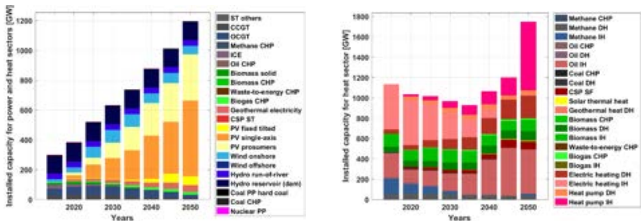
Figure 3.10-8: South America – Technology-wise installed capacities for power (left) and heat (right) during the energy transition from 2015 to 2050.
