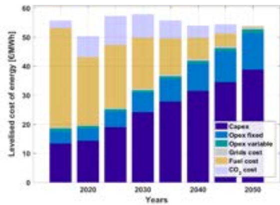
Figure 3.1-7: Global – Capital costs for five-year intervals (left) and levelised cost of energy (right) during the energy transition from 2015 to 2050.
