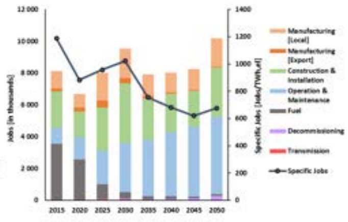
Figure 3.7-33: Northeast Asia – Jobs created by various power generation and storage technologies (left) and jobs created based on different categories with the development of electricity demand specific jobs (right) during the energy transition from 2015 to 2050.
