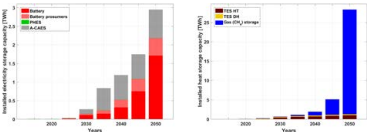
Figure 3.5-10: Sub-Saharan Africa – Installed electricity storage capacities (left) and heat storage capacities (right) during the energy transition from 2015 to 2050.
