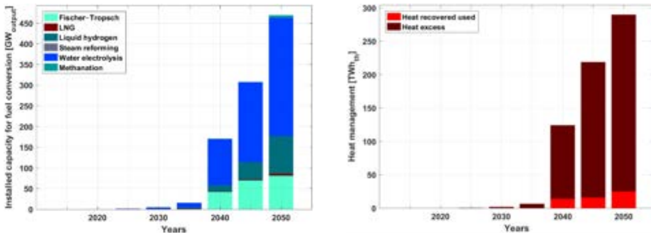
Figure 3.3-17: Eurasia – Transport sector installed capacity for fuel conversion (left) and heat management (right) during the energy transition from 2015 to 2050.
