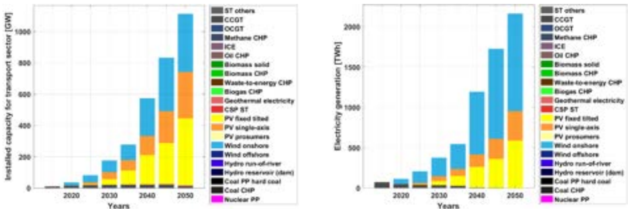
Figure 3.3-15: Eurasia – Transport sector installed power generation capacity (left) and electricity generation (right) during the energy transition from 2015 to 2050.
