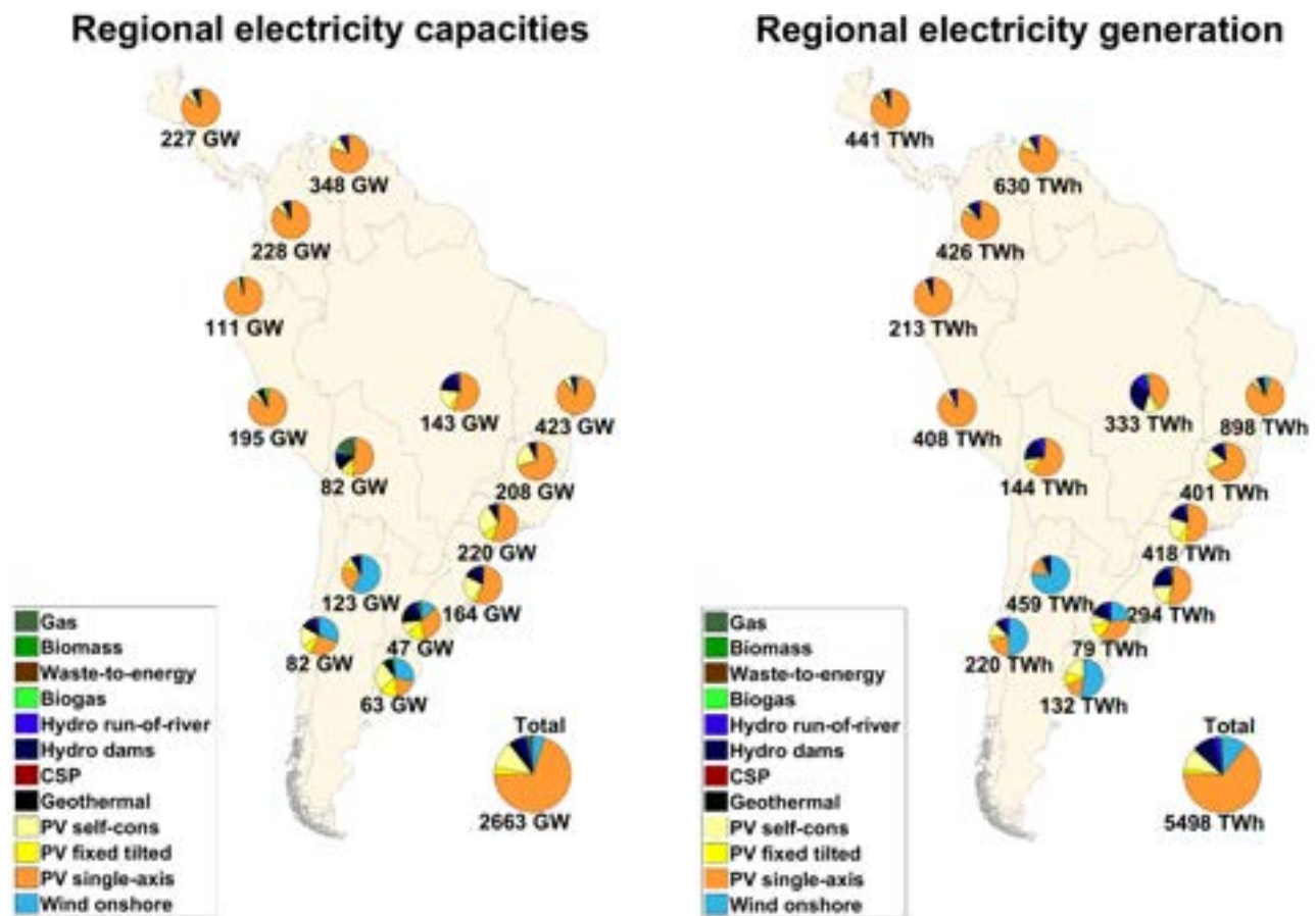
Figure 3.10-25: South America – Regional electricity generation capacities (left) and electricity generation (right) in 2050.
