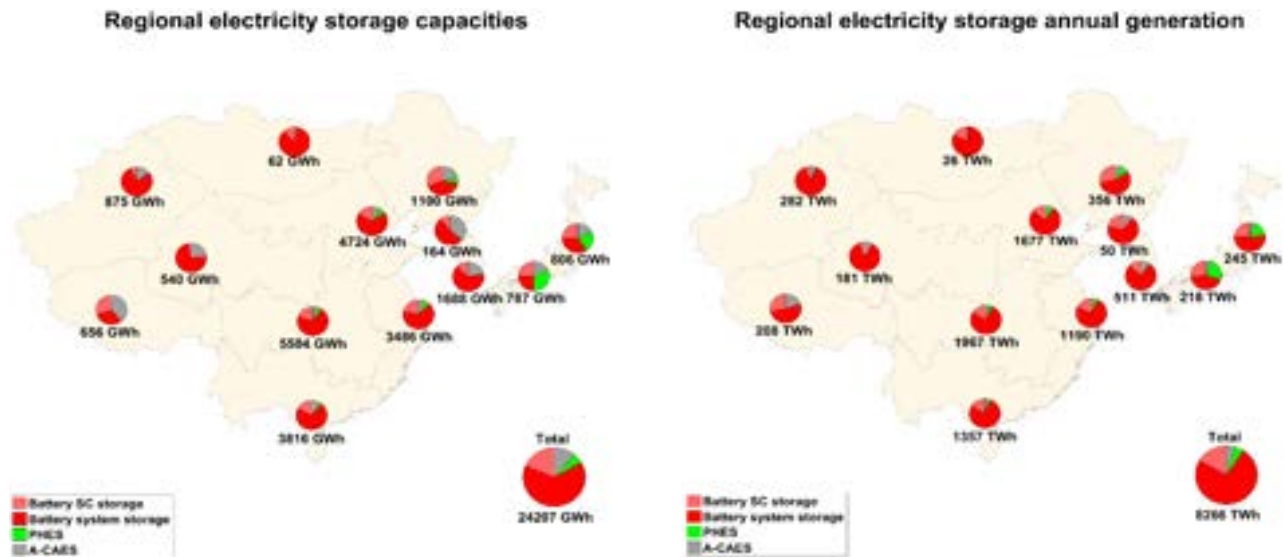
Figure 3.7-28: Northeast Asia – Regional electricity storage capacities (left) and electricity storage annual throughput (right) in 2050.
