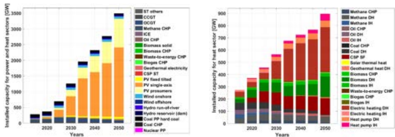
Figure 3.8-8: Southeast Asia – Technology-wise installed capacities for power (left) and heat (right) during the energy transition from 2015 to 2050.
