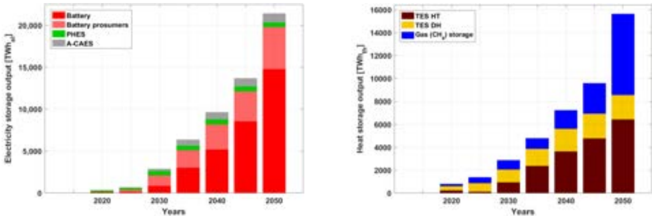
Figure 3.1-11: Global – Electricity storage output (left) and heat storage output (right) during the energy transition from 2015 to 2050.
