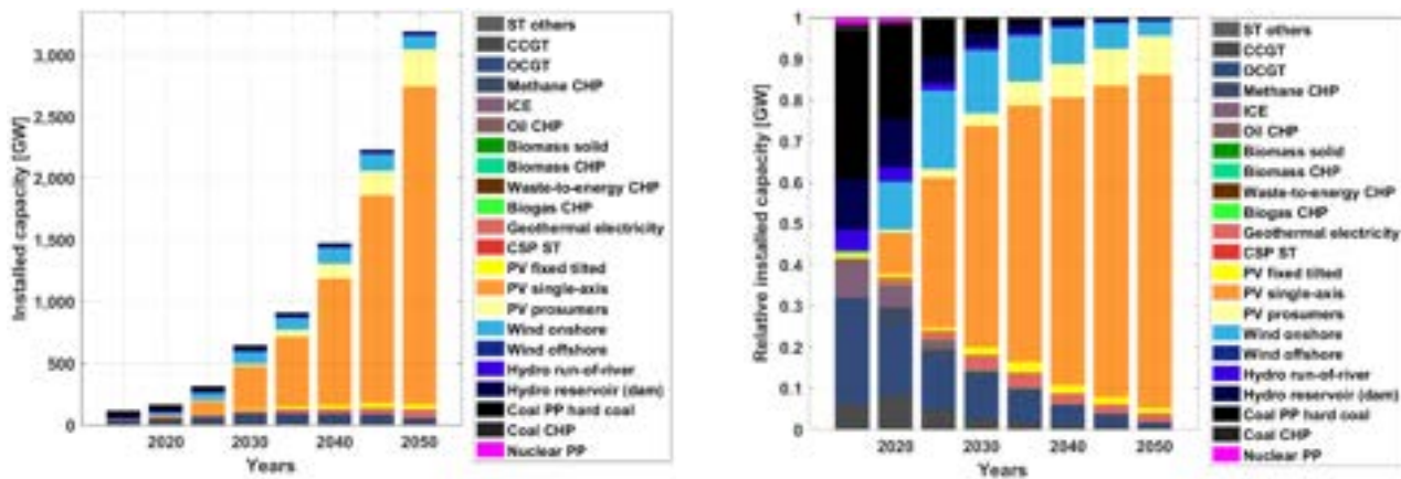
Figure 3.5-2: Sub-Saharan Africa – Technology-wise installed capacities (left) and technology-wise shares of installed capacities (right) during the energy transition from 2015 to 2050.
