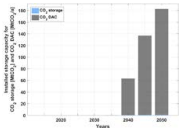
Figure 3.5-18: Sub-Saharan Africa – Transport sector installed capacity for gas (methane and hydrogen) storage (left) and CO 2 direct air capture and CO 2 storage (right) during the energy transition from 2015 to 2050.
