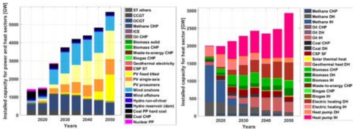
Figure 3.9-8: North America – Technology-wise installed capacities for power (left) and heat (right) during the energy transition from 2015 to 2050.
