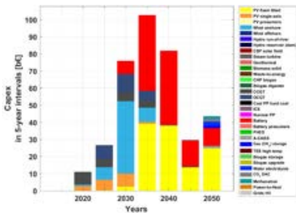
Figure 3.4-24: MENA – Capital costs for five-year intervals (left) and levelised cost of water (right) during the energy transition from 2015 to 2050.
