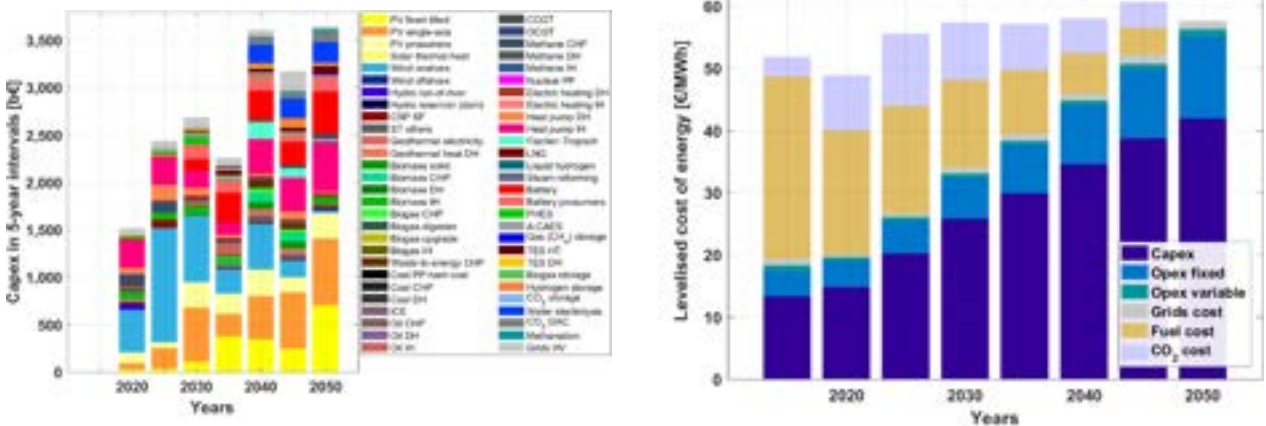
Figure 3.7-7: Northeast Asia – Capital costs for five-year intervals (left) and levelised cost of energy (right) during the energy transition from 2015 to 2050.
