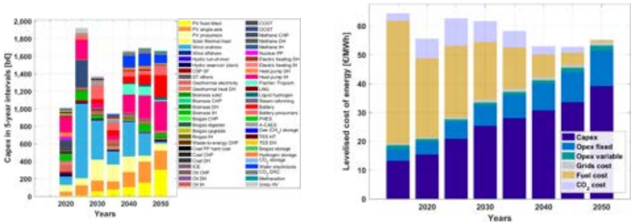
Figure 3.9-7: North America – Capital costs for five-year intervals (left) and levelised cost of energy (right) during the energy transition from 2015 to 2050.
