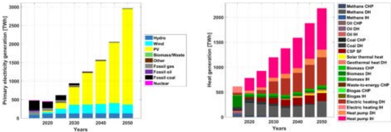
Figure 3.5-9: Sub-Saharan Africa – Primary electricity generation (left) and technology-wise heat generation (right) during the energy transition from 2015 to 2050.
