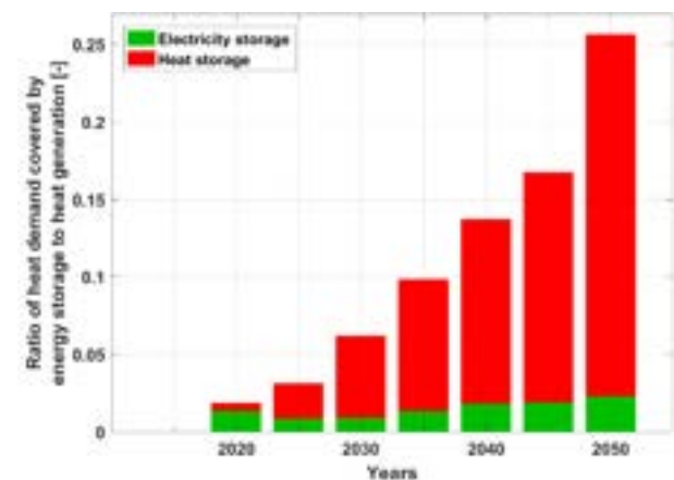
Figure 3.1-5: Global – Heat demand covered by energy storage (left) and the ratio of heat demand covered by different forms of energy storage (right) during the energy transition from 2015 to 2050.
