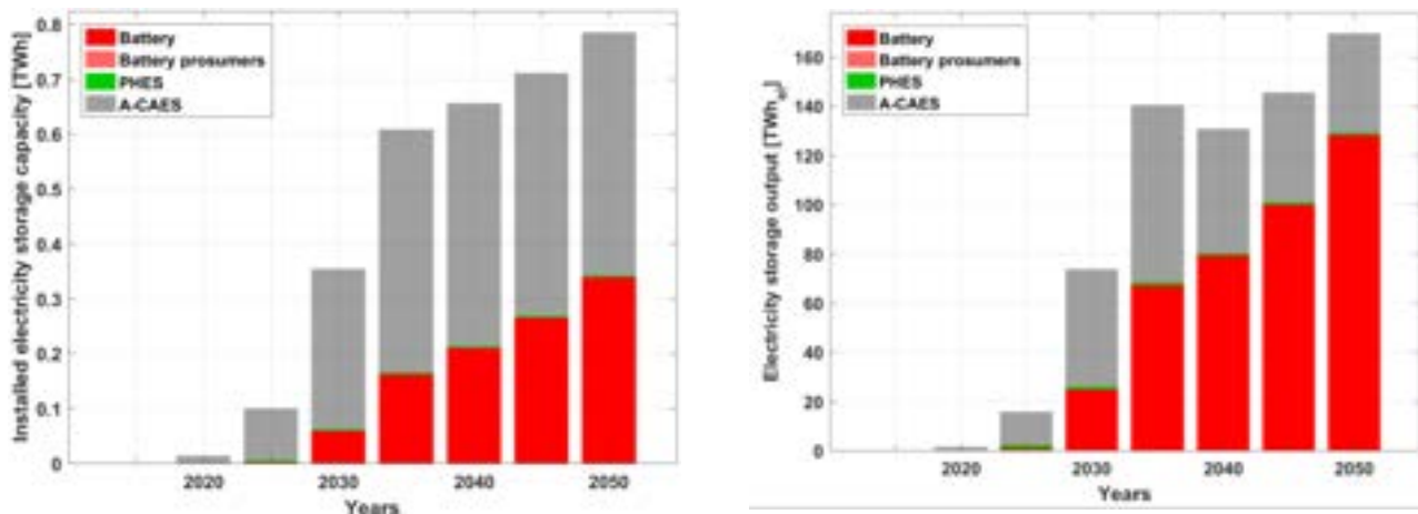
Figure 3.3-16: Eurasia – Transport sector installed electricity storage capacity (left) and electricity storage output (right) during the energy transition from 2015 to 2050.
