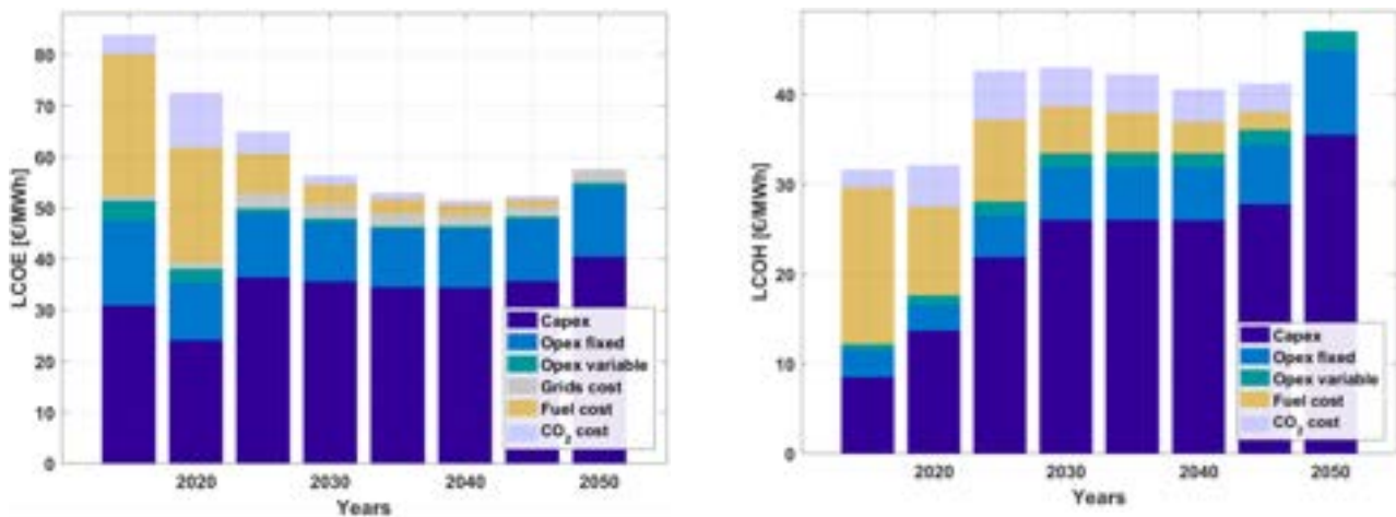
Figure 3.3-12: Levelised cost of electricity (left) and levelised cost of heat (right) during the energy transition from 2015 to 2050 in Europe.
