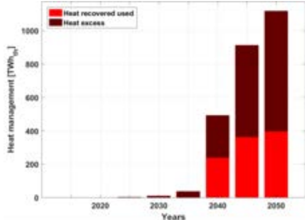
Figure 3.9-17: North America – Transport sector installed capacity for fuel conversion (left) and heat management (right) during the energy transition from 2015 to 2050.
