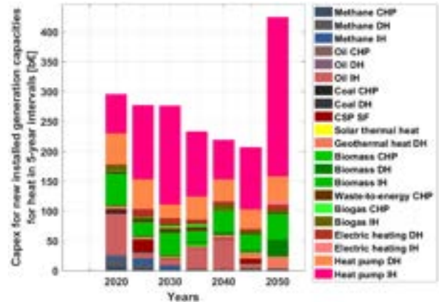
Figure 3.2-13: Europe – Capital costs of installed generation capacities in five-year intervals for electricity (left) and heat (right) during the energy transition from 2015 to 2050.
