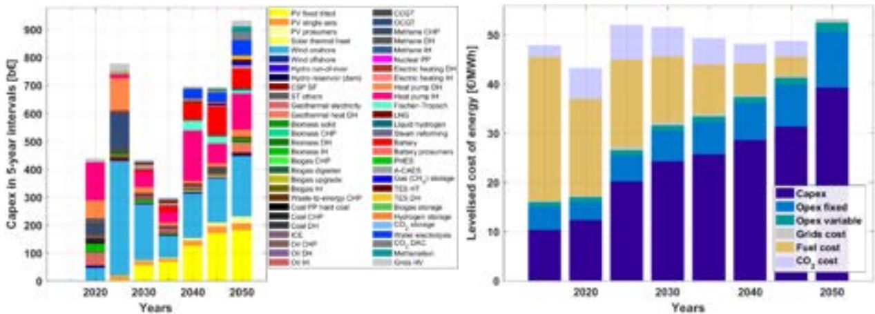
Figure 3.3-7: Eurasia – Capital costs for five-year intervals (left) and levelised cost of energy (right) during the energy transition from 2015 to 2050.
