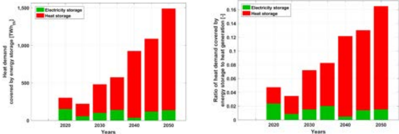
Figure 3.9-5: North America – Heat demand covered by energy storage (left) and the ratio of heat demand covered by different forms of energy storage (right) during the energy transition from 2015 to 2050.
