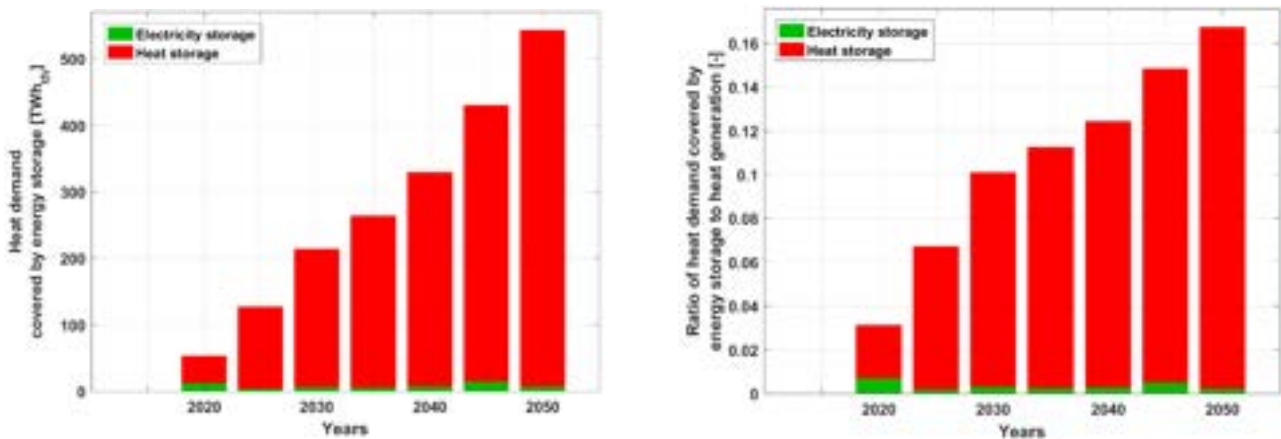
Figure 3.10-5: South America – Heat demand covered by energy storage (left) and the ratio of heat demand covered by different forms of energy storage (right) during the energy transition from 2015 to 2050.
