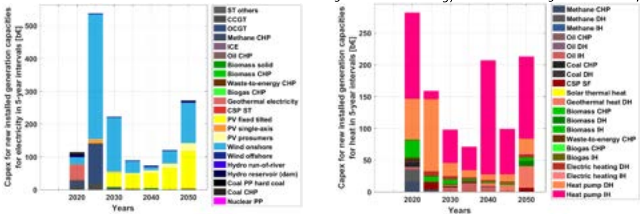
Figure 3.3-13: Eurasia – Capital costs of installed generation capacities in five-year intervals for electricity (left) and heat (right) during the energy transition from 2015 to 2050.
